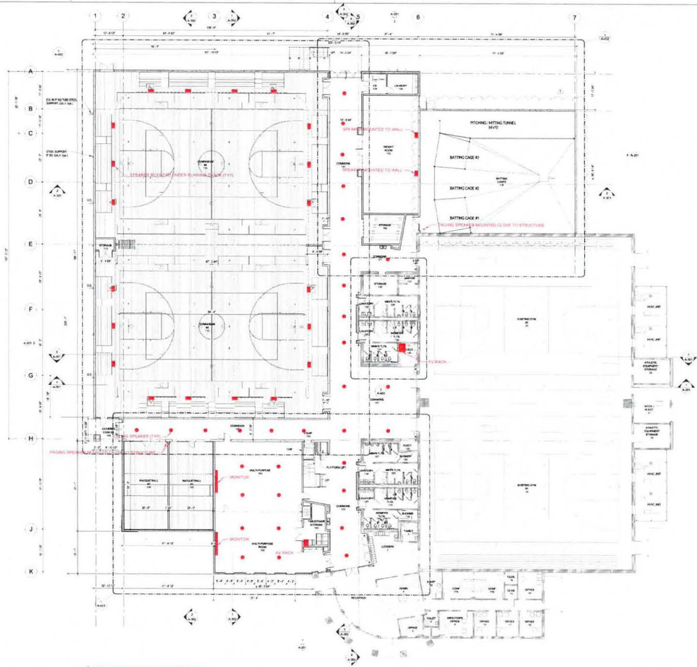
1 SCHEDULED EQUIPMENT LAYOUT - FIRST FLOOR - NOT TO SCALE
