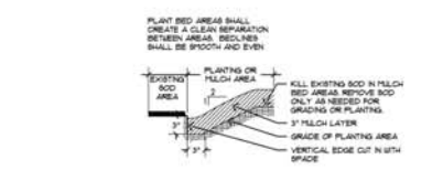
3 Plant Bed Edge Detail Against Sod Not to Scale
